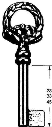
M = 23,33 mm AD = 23,33,45 mm
